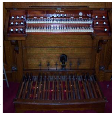
Möller Console
